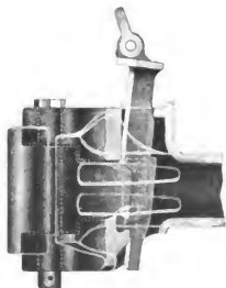
Fig. 3972. R. E. Janney Coupler, Unlocked.
